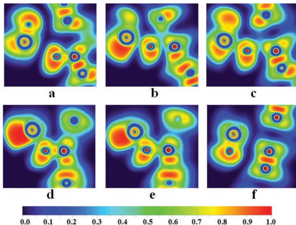
Fig. 4 The two-dimensional electron localization function (ELF) color-filled maps of \text{SO}_2 reacting with the oxygen-functionalized graphene sheet: (a–c) the ELF maps of the reactant complex, first transition state, and intermediate in the \text{C1-O1-S} plane; (d–f) the ELF maps of the intermediate, second transition state, and product complex in the \text{C2-O1-S} plane. Areas beyond the interaction are omitted for clarity.
