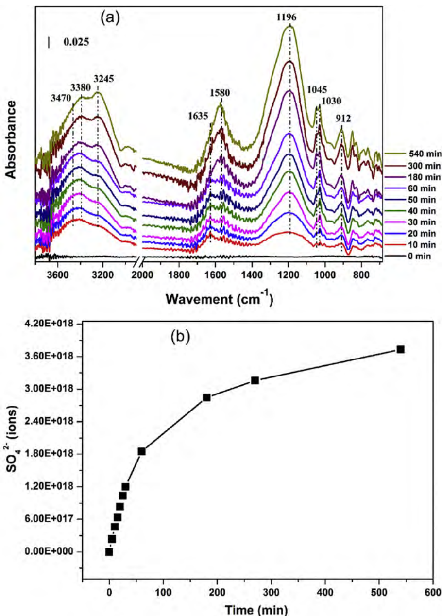
Fig. 1. (a) Dynamic changes in the ATR-IR spectra of soot as a function of time. (b) Sulfate formation on soot as a function of time during the reaction with \text{SO}_2 . ATR-IR reaction conditions: total flow rate of 100 \text{ mL min}^{-1} , 5 \text{ ppmv SO}_2 + zero air, soot with fuel/oxygen ratio of 0.134, RH of 54%, temperature of 298 K.
